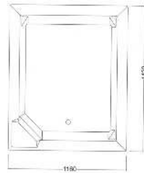
LA-121468 Size:1160×1420×680mm Capacity:530L
